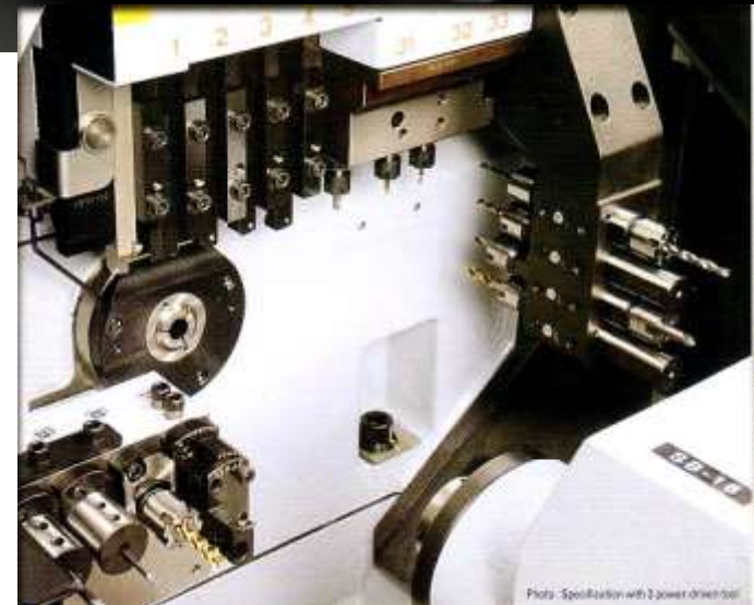
Photo: Specification with 2 power driver tool
